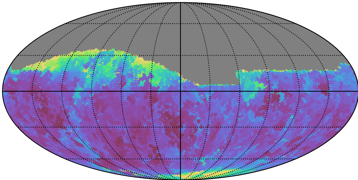
noroll_mjdp60_v3.4_10yrs Yr 1 z band: Min seeingEff
