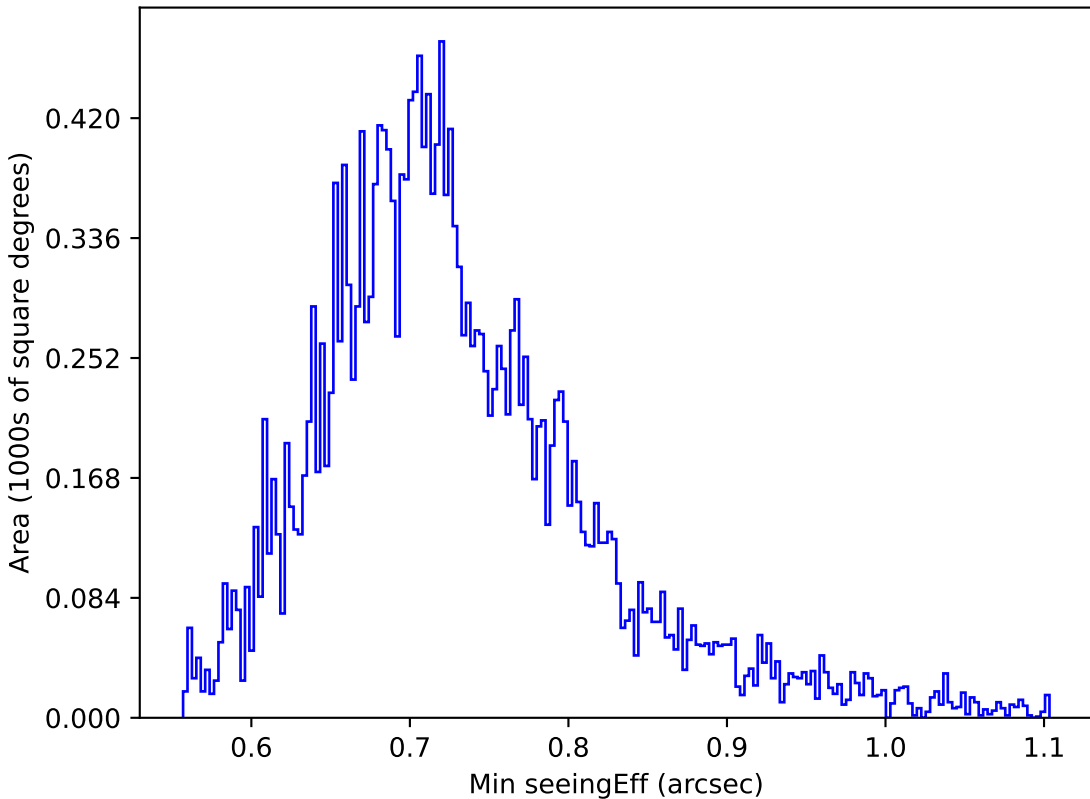
noroll_mjdp60_v3.4_10yrs Yr 1 y band: Min seeingEff
