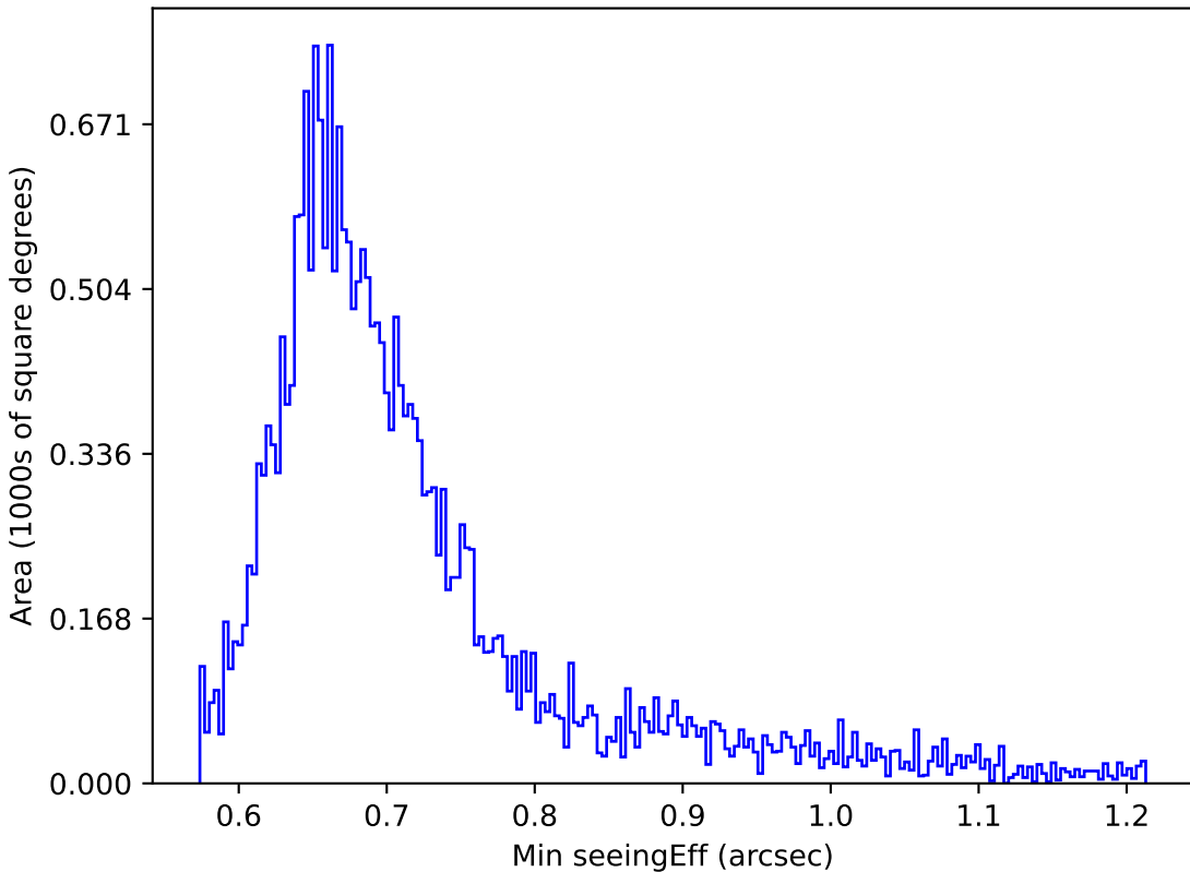
noroll_mjdp60_v3.4_10yrs Yr 1 i band: Min seeingEff
