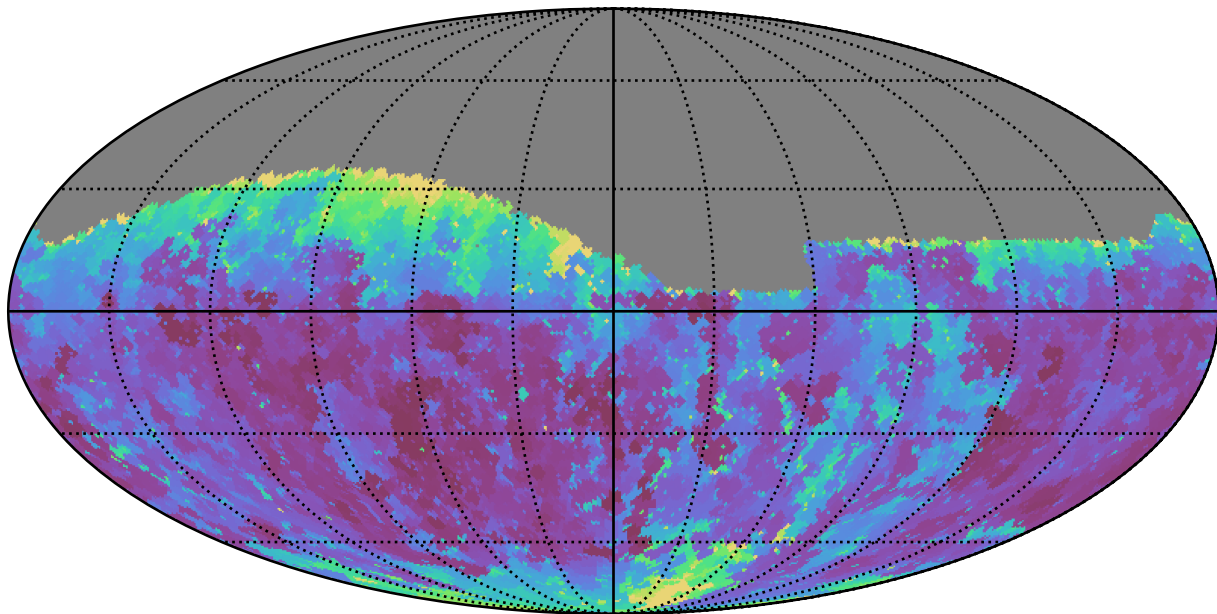
noroll_mjdp60_v3.4_10yrs Yr 1 g band: Min seeingEff
