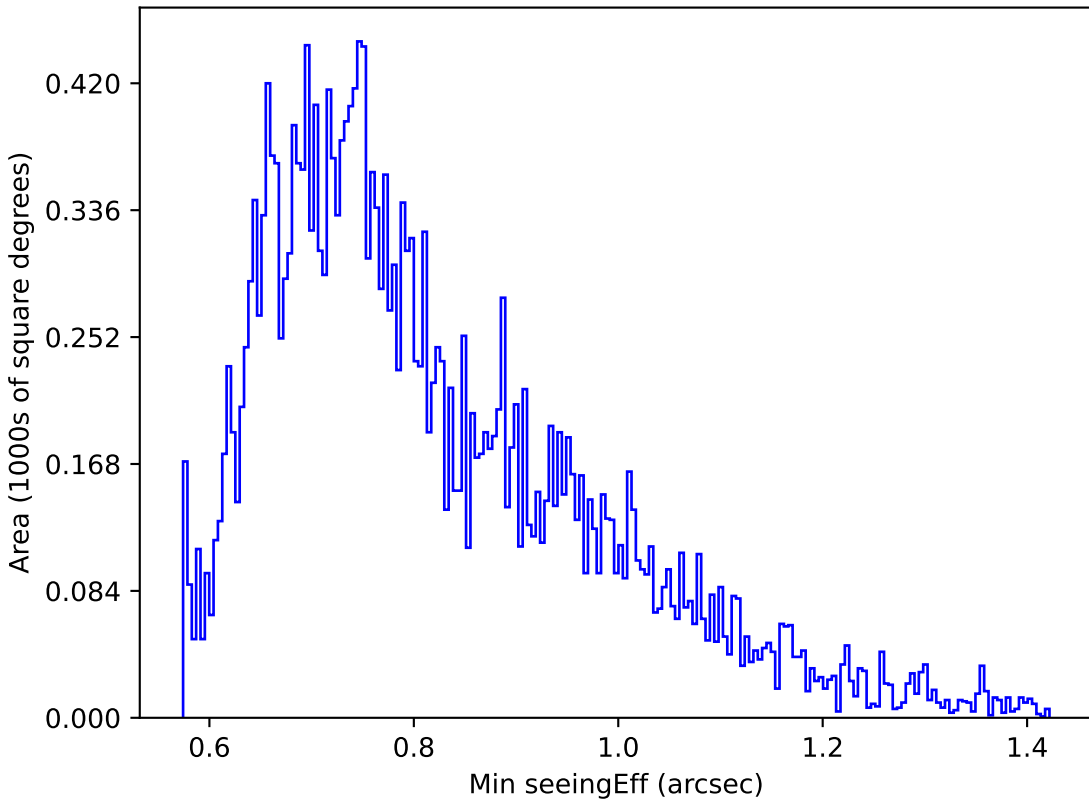
noroll_mjdp60_v3.4_10yrs Yr 1 g band: Min seeingEff
