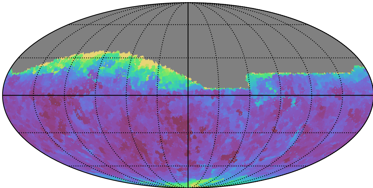
noroll_mjdp60_v3.4_10yrs Yr 1 all bands: Min seeingEff
