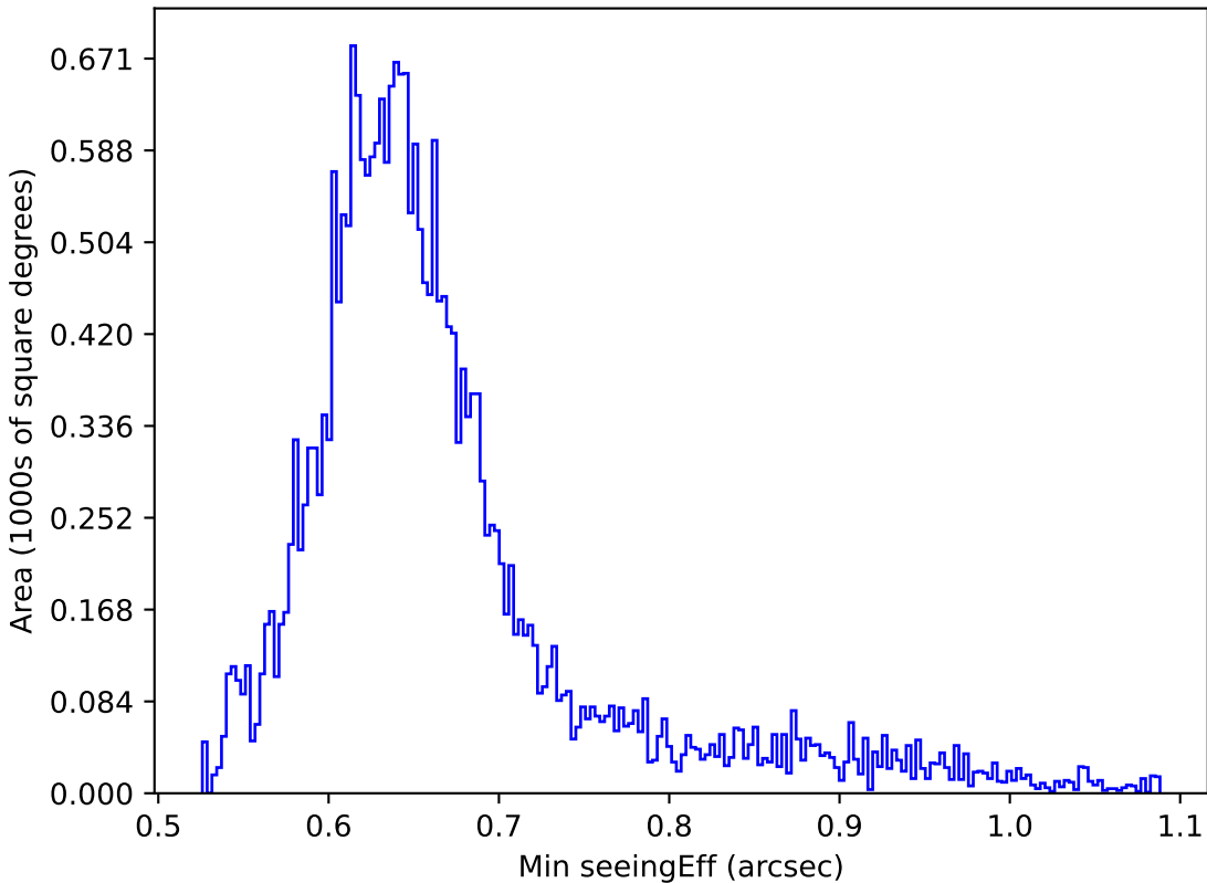
noroll_mjdp60_v3.4_10yrs Yr 1 all bands: Min seeingEff
