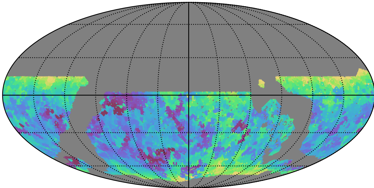
noroll_mjdp60_v3.4_10yrs WFD z band: Min seeingEff
