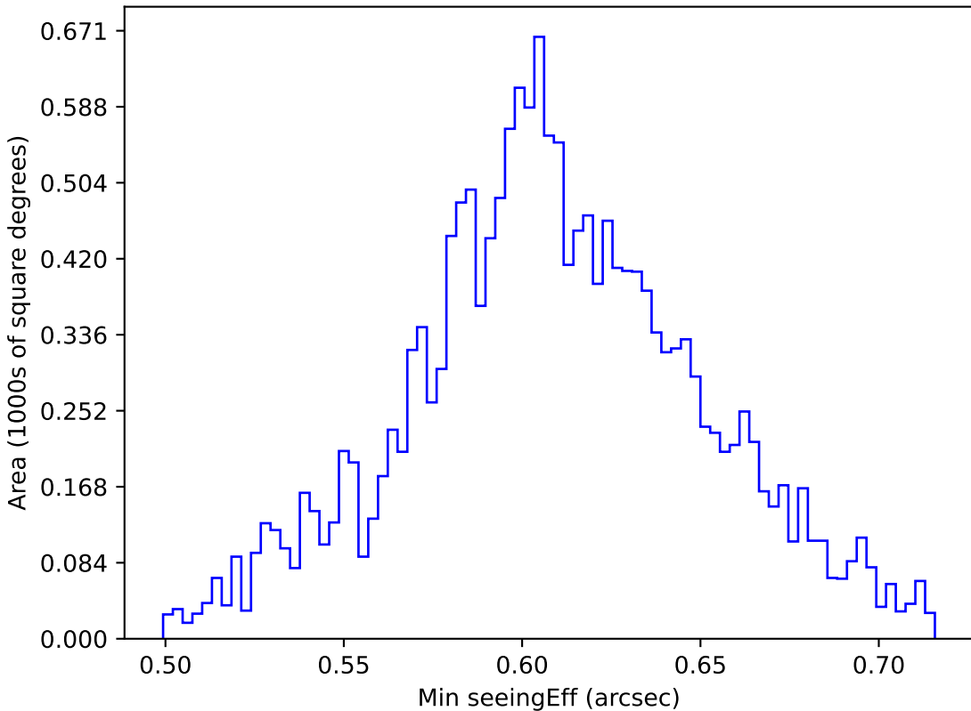
noroll_mjdp60_v3.4_10yrs WFD z band: Min seeingEff
