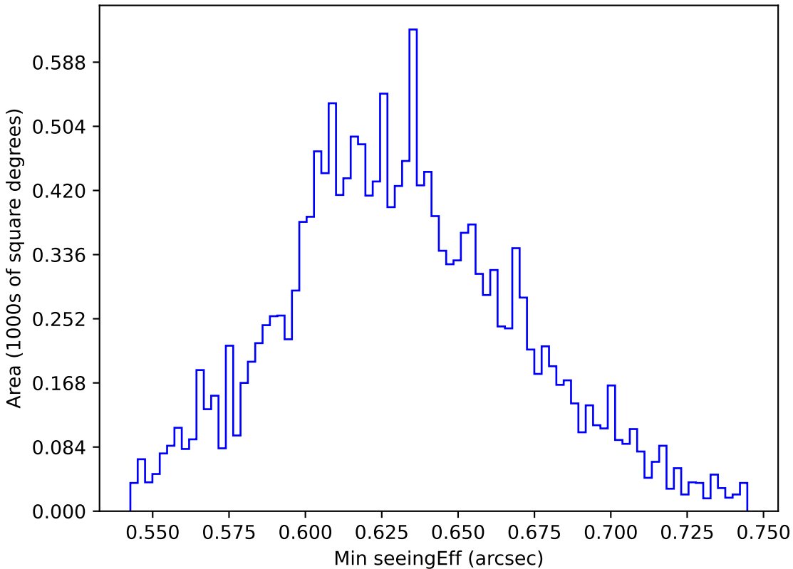
noroll_mjdp60_v3.4_10yrs WFD y band: Min seeingEff
