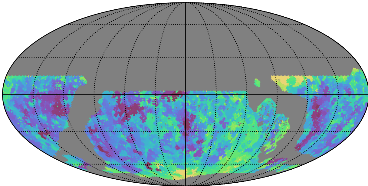
noroll_mjdp60_v3.4_10yrs WFD u band: Min seeingEff
