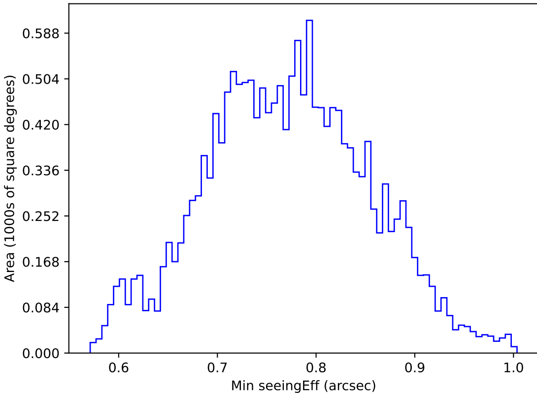
noroll_mjdp60_v3.4_10yrs WFD u band: Min seeingEff
