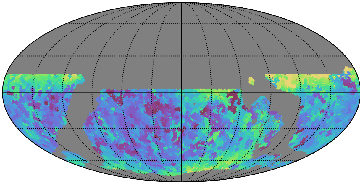
noroll_mjdp60_v3.4_10yrs WFD r band: Min seeingEff
