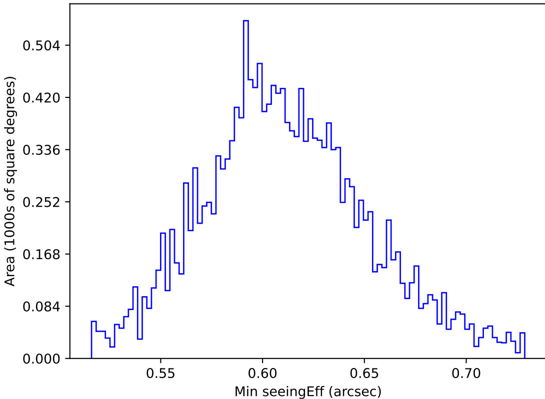
noroll_mjdp60_v3.4_10yrs WFD r band: Min seeingEff
