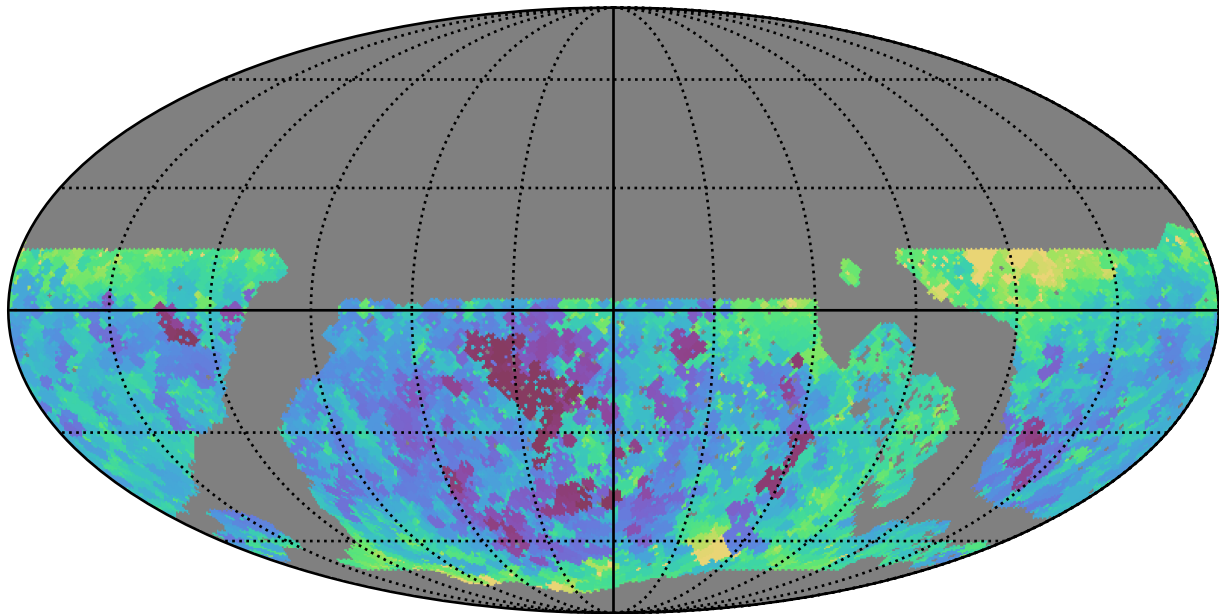
noroll_mjdp60_v3.4_10yrs WFD g band: Min seeingEff
