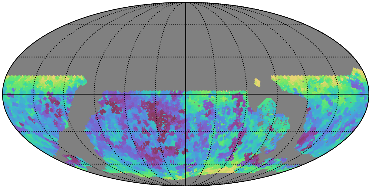
noroll_mjdp60_v3.4_10yrs WFD all bands: Min seeingEff
