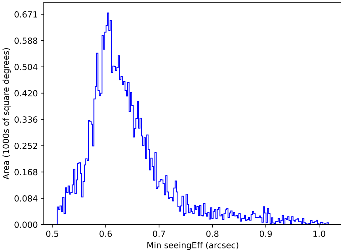
noroll_mjdp60_v3.4_10yrs All sky z band: Min seeingEff
