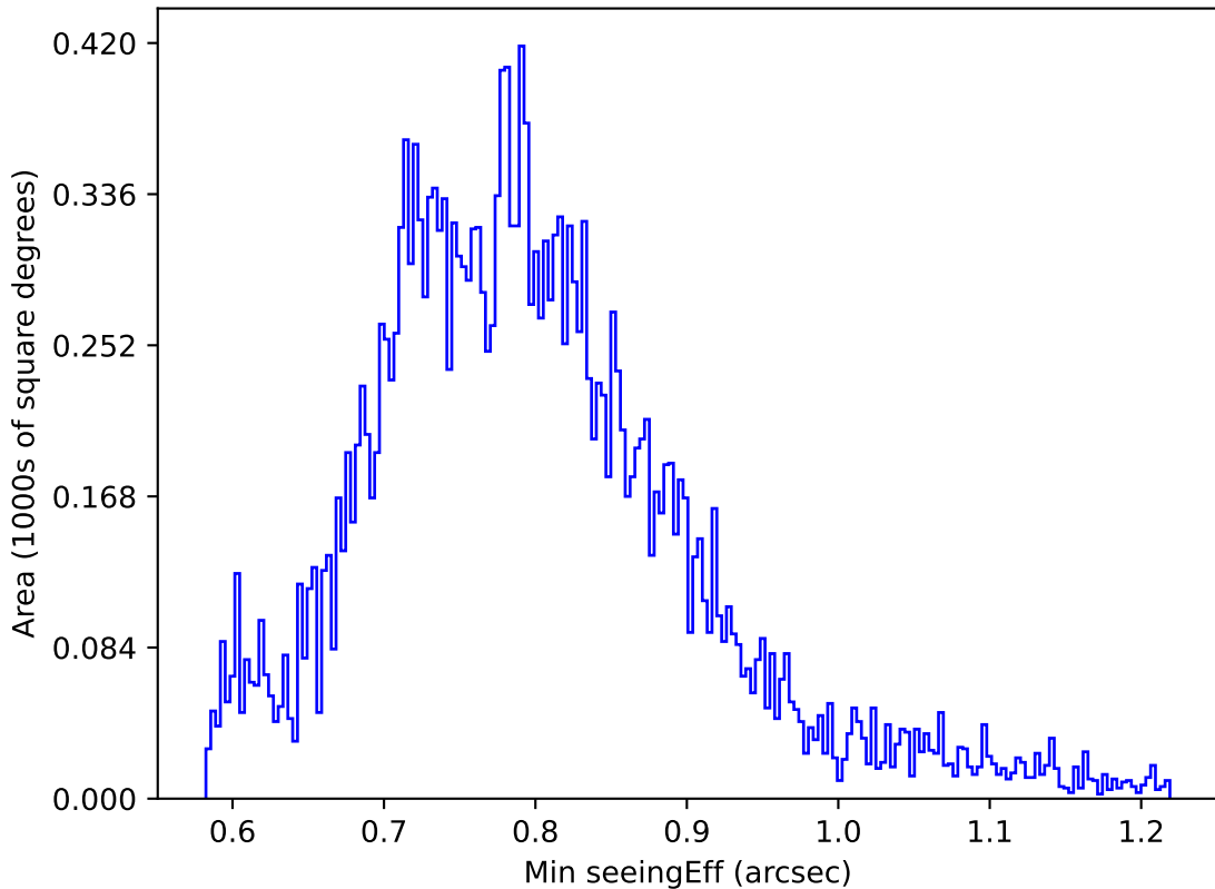
noroll_mjdp60_v3.4_10yrs All sky u band: Min seeingEff
