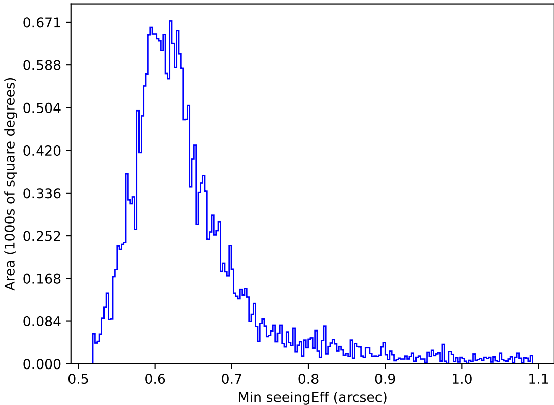
noroll_mjdp60_v3.4_10yrs All sky r band: Min seeingEff
