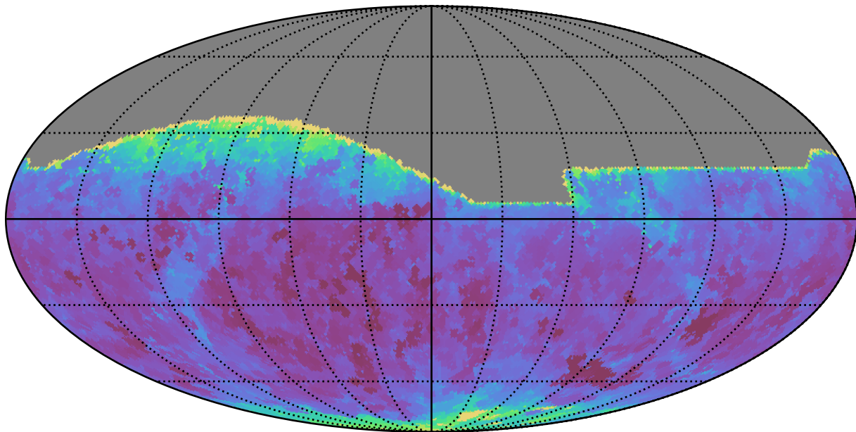
noroll_mjdp60_v3.4_10yrs All sky i band: Min seeingEff
