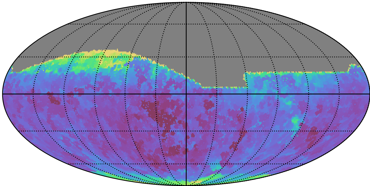
noroll_mjdp60_v3.4_10yrs All sky g band: Min seeingEff
