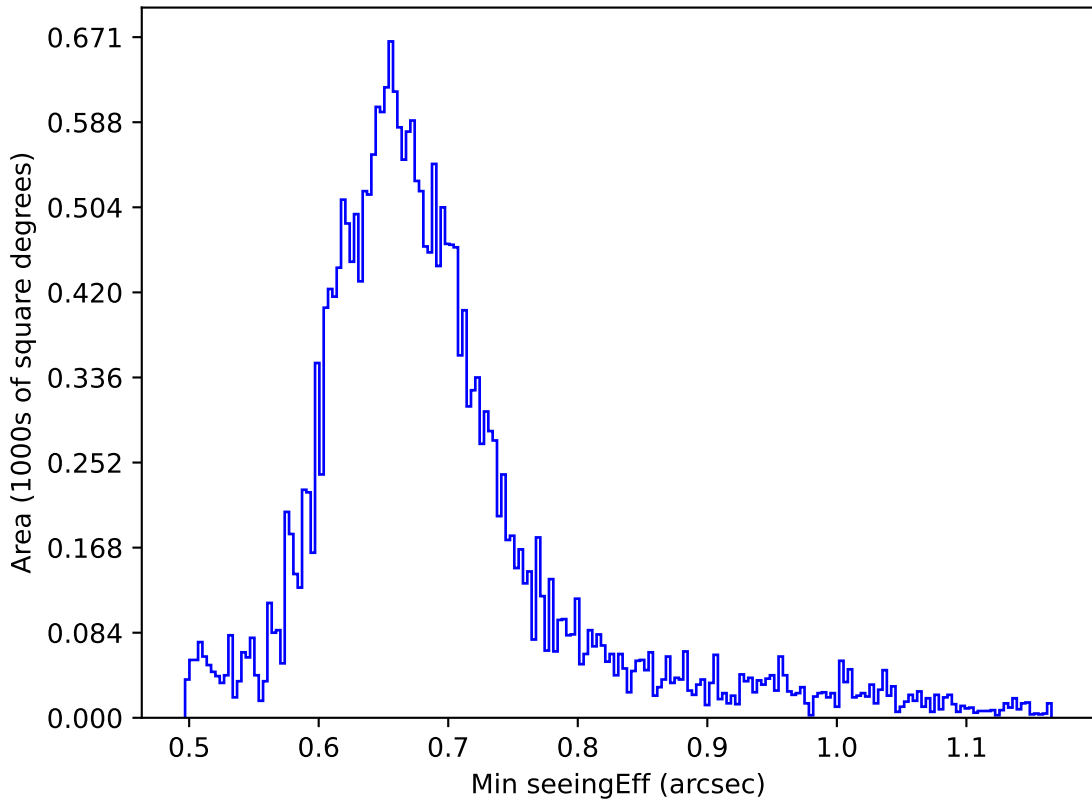
noroll_mjdp60_v3.4_10yrs All sky g band: Min seeingEff
