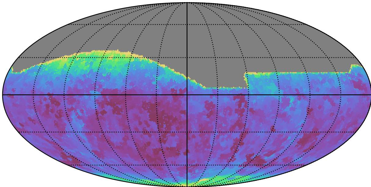
noroll_mjdp60_v3.4_10yrs All sky all bands: Min seeingEff
