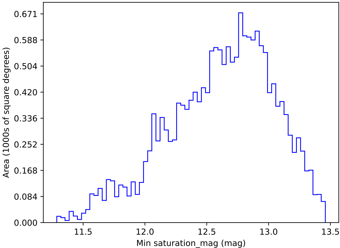
noroll_mjdp60_v3.4_10yrs WFD r band: Min saturation_mag
