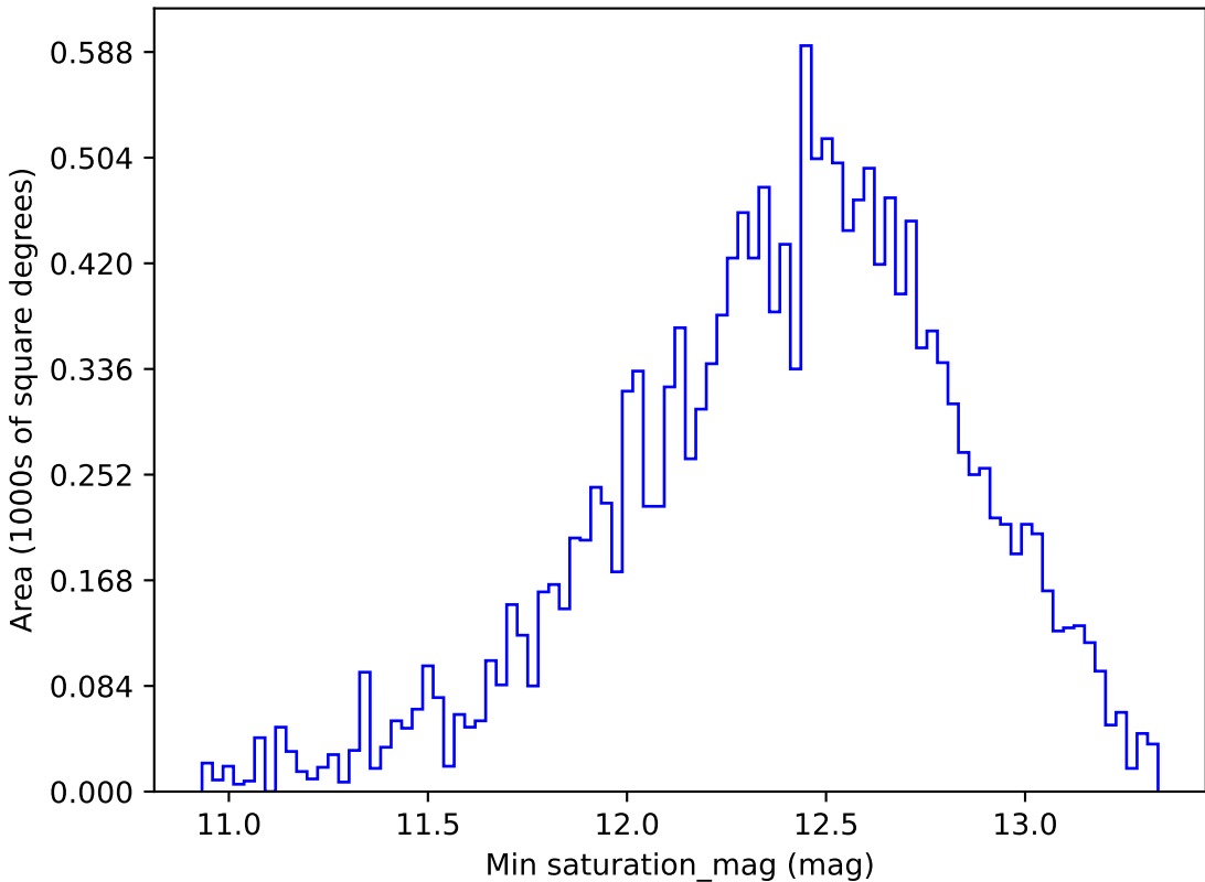
noroll_mjdp60_v3.4_10yrs WFD i band: Min saturation_mag
