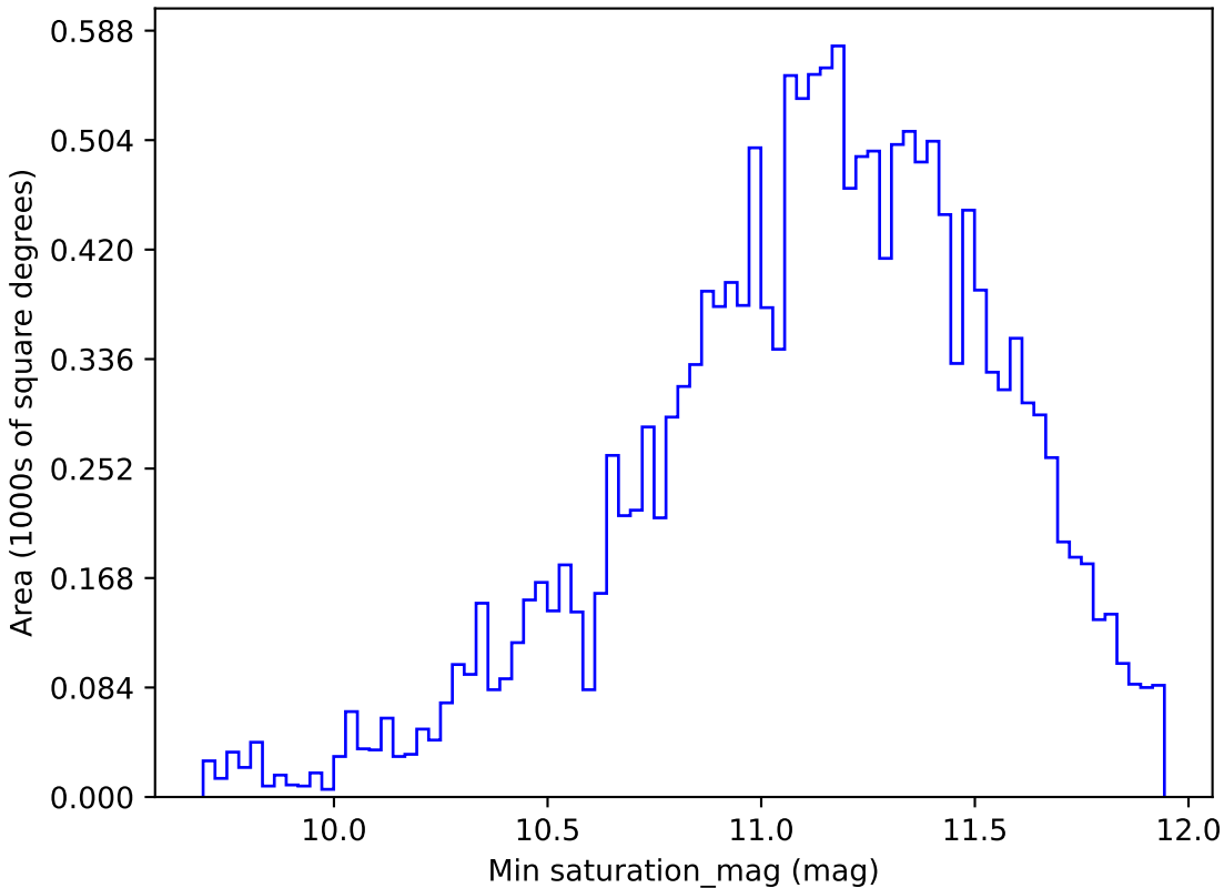
noroll_mjdp60_v3.4_10yrs WFD all bands: Min saturation_mag
