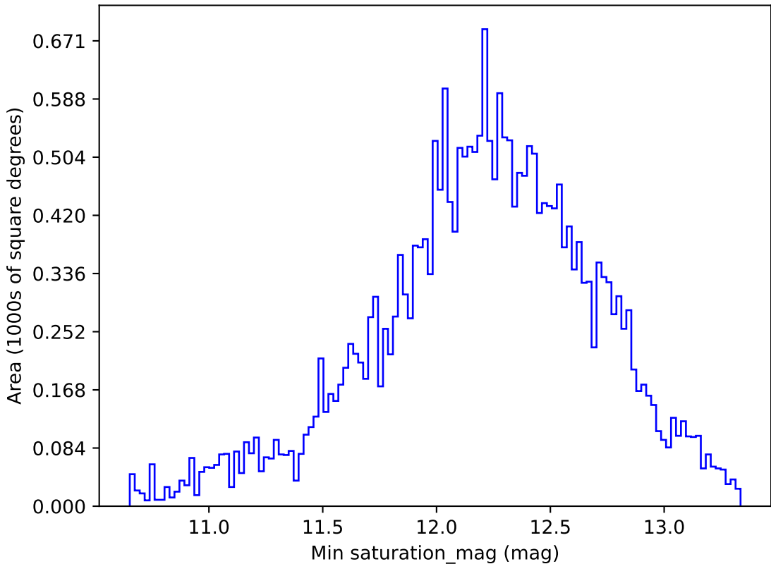
noroll_mjdp60_v3.4_10yrs All sky z band: Min saturation_mag
