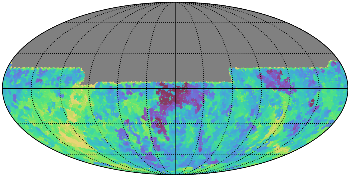
noroll_mjdp60_v3.4_10yrs All sky y band: Min saturation_mag
