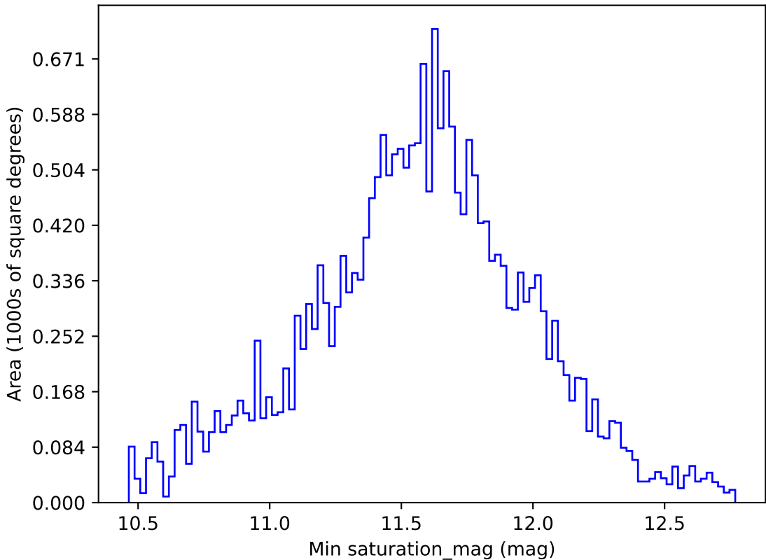
noroll_mjdp60_v3.4_10yrs All sky u band: Min saturation_mag
