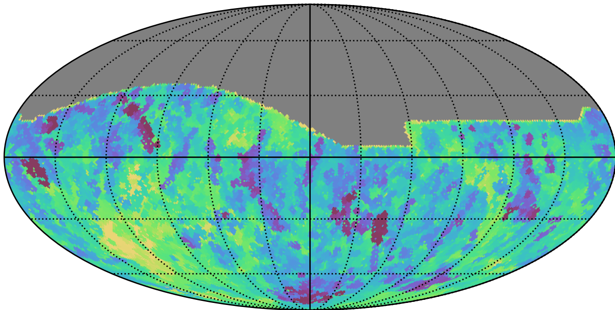
noroll_mjdp60_v3.4_10yrs All sky i band: Min saturation_mag
