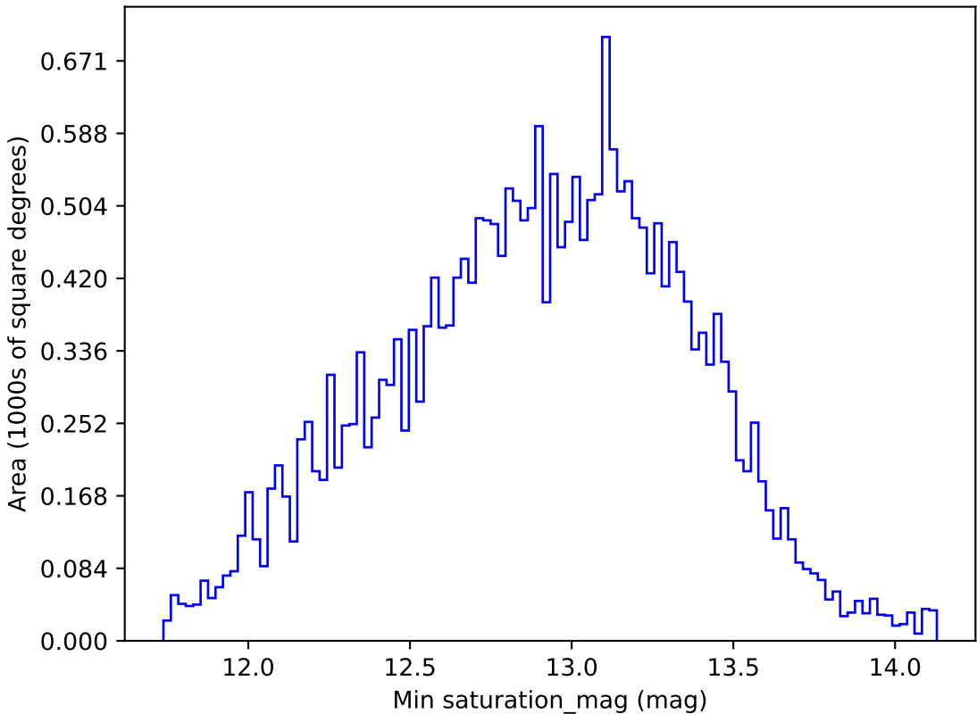
noroll_mjdp60_v3.4_10yrs All sky g band: Min saturation_mag
