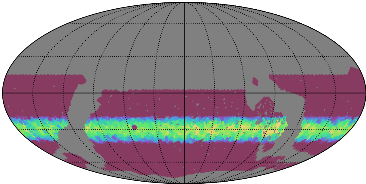
noroll_mjdp60_v3.4_10yrs WFD z band: Min normairmass
