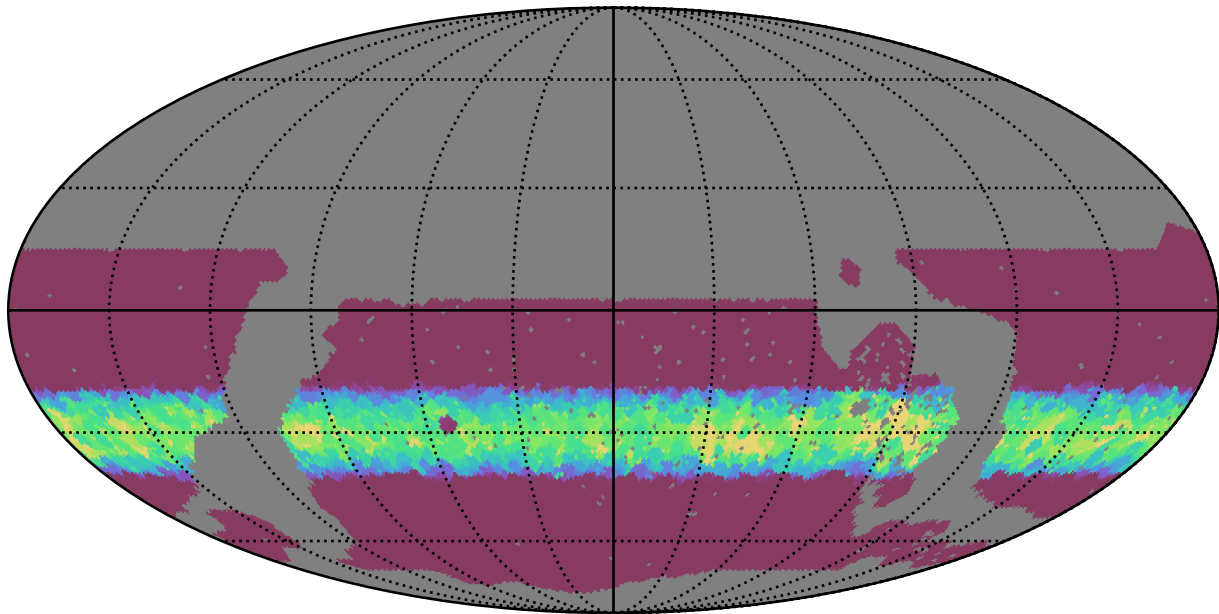
noroll_mjdp60_v3.4_10yrs WFD y band: Min normairmass
