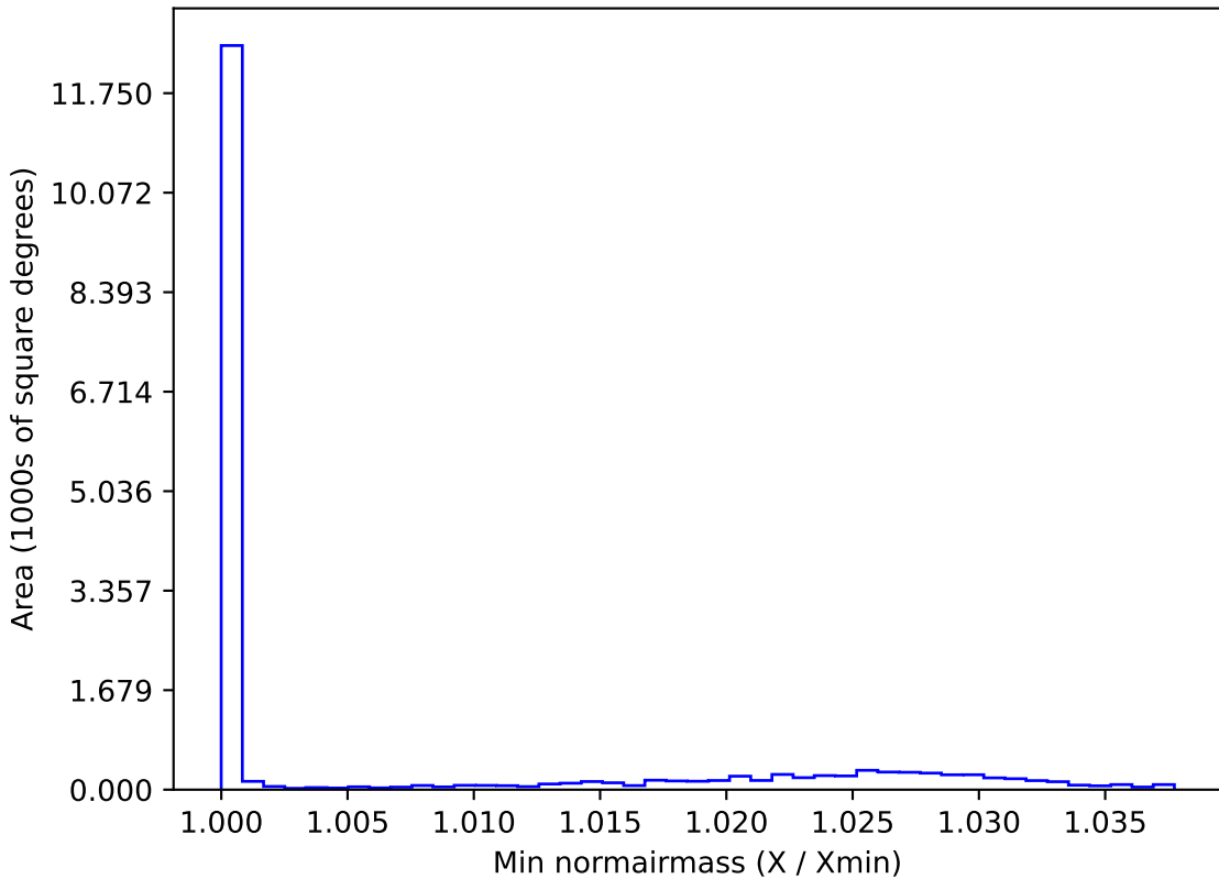
noroll_mjdp60_v3.4_10yrs WFD y band: Min normairmass
