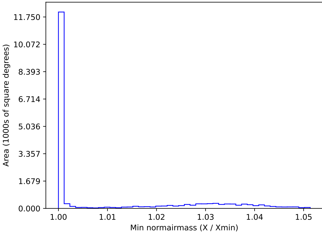
noroll_mjdp60_v3.4_10yrs WFD u band: Min normairmass
