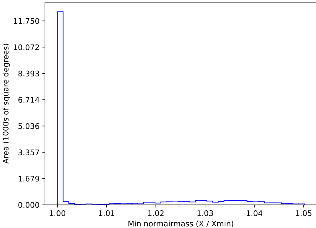
noroll_mjdp60_v3.4_10yrs WFD g band: Min normairmass
