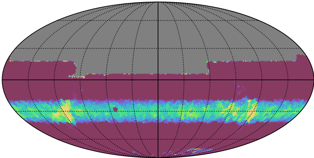
noroll_mjdp60_v3.4_10yrs All sky y band: Min normairmass
