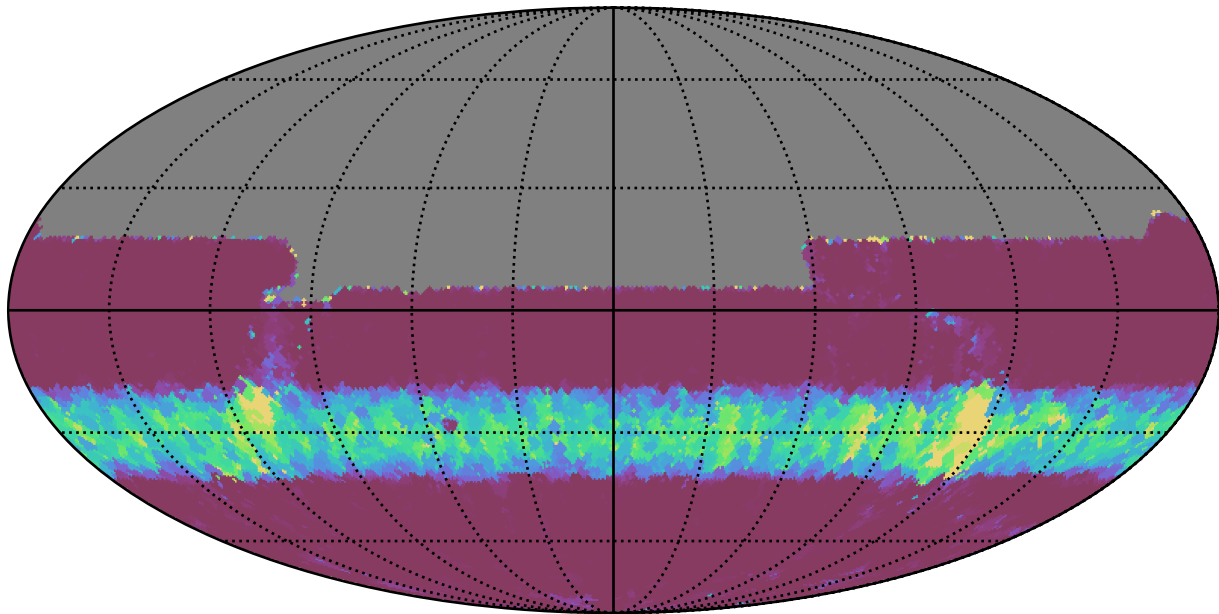
noroll_mjdp60_v3.4_10yrs All sky u band: Min normairmass
