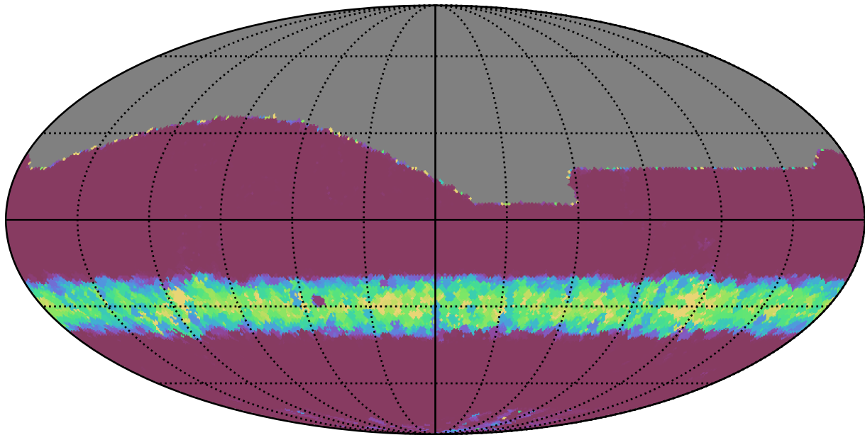
noroll_mjdp60_v3.4_10yrs All sky r band: Min normairmass
