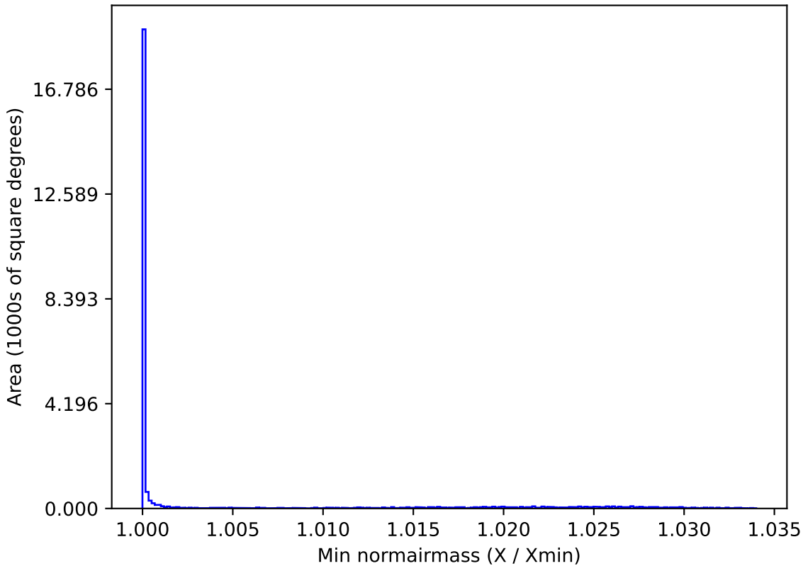
noroll_mjdp60_v3.4_10yrs All sky r band: Min normairmass
