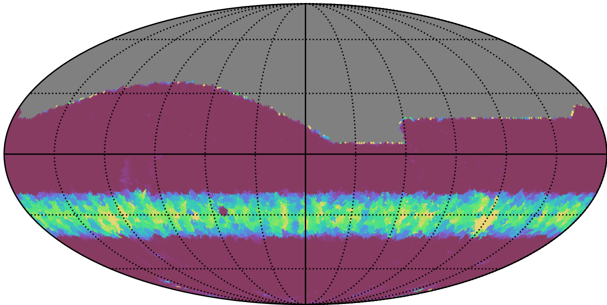
noroll_mjdp60_v3.4_10yrs All sky g band: Min normairmass
