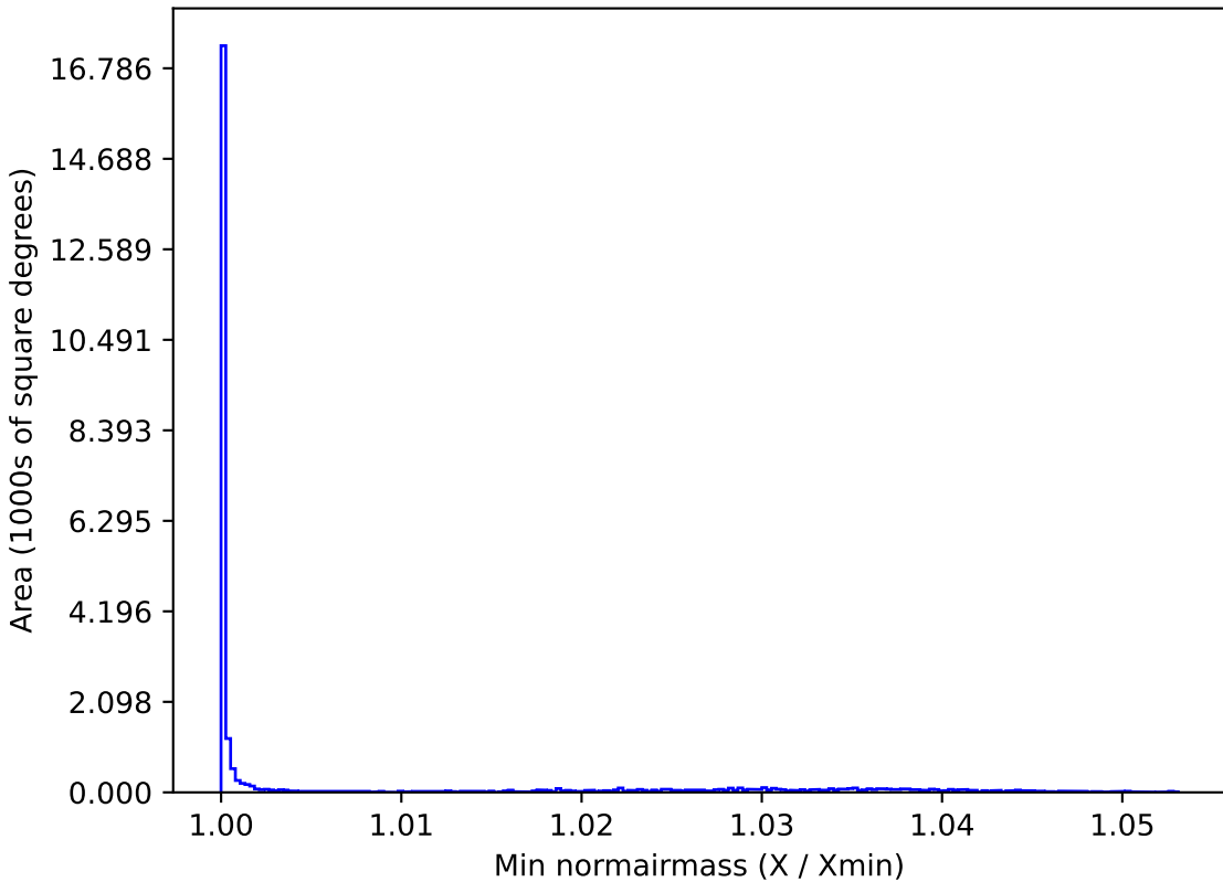
noroll_mjdp60_v3.4_10yrs All sky g band: Min normairmass
