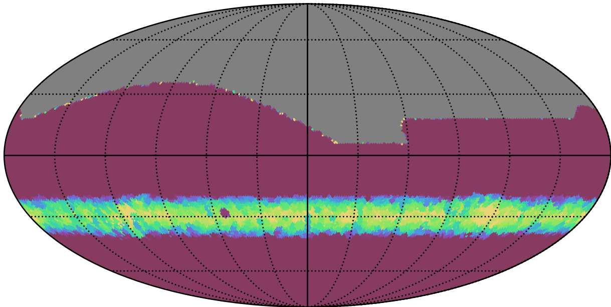
noroll_mjdp60_v3.4_10yrs All sky all bands: Min normairmass
