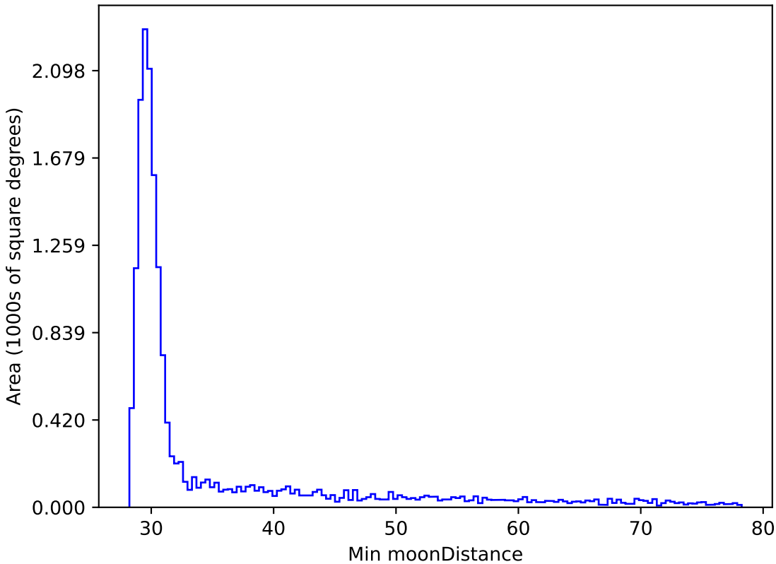
noroll_mjdp60_v3.4_10yrs WFD z band: Min moonDistance
