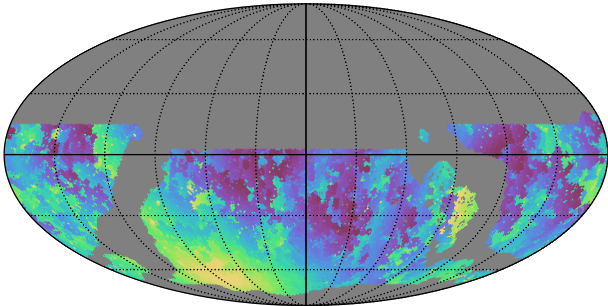
noroll_mjdp60_v3.4_10yrs WFD u band: Min moonDistance
