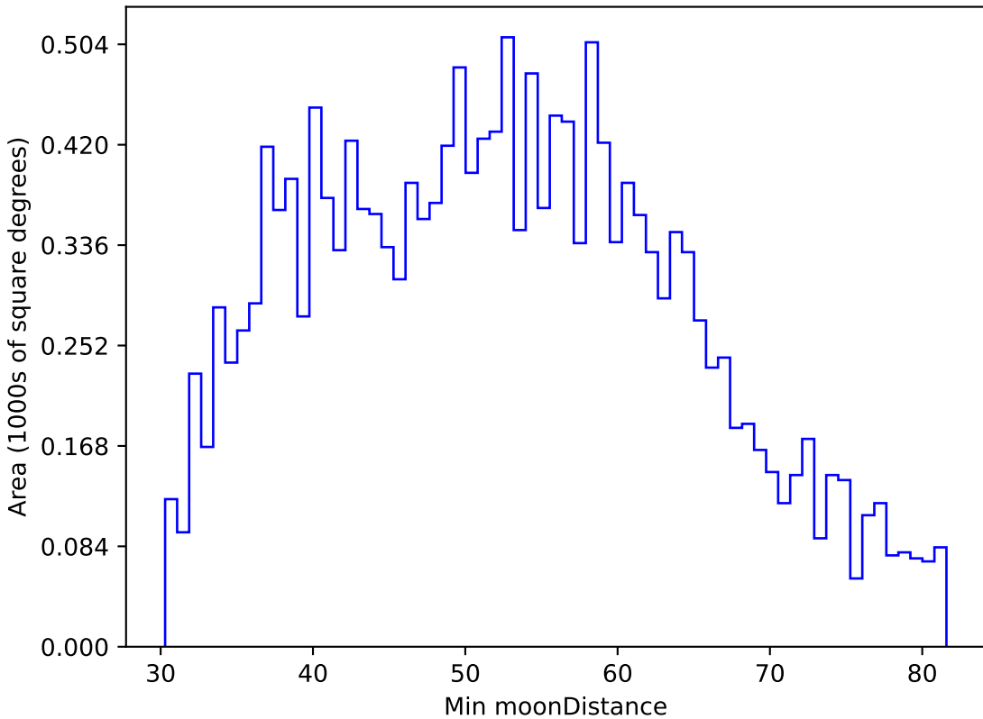
noroll_mjdp60_v3.4_10yrs WFD u band: Min moonDistance
