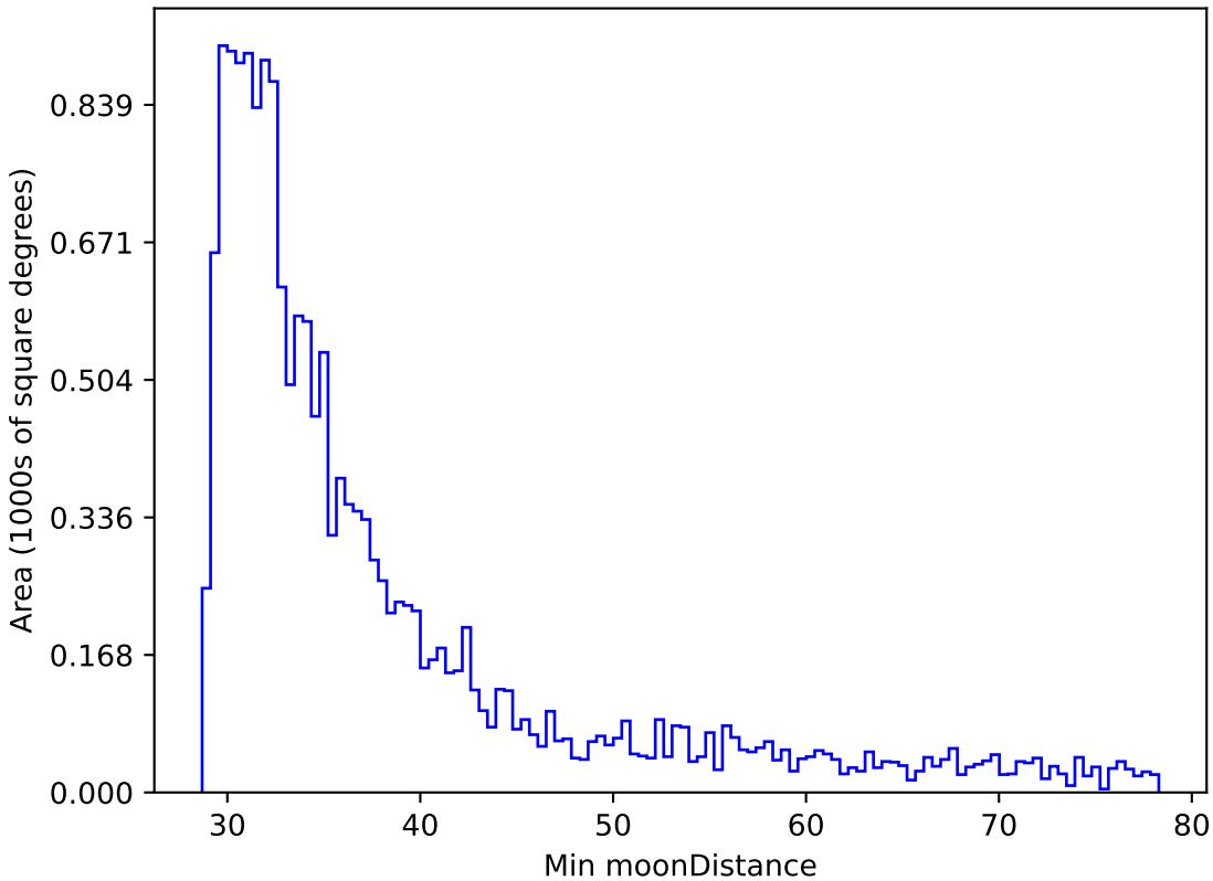
noroll_mjdp60_v3.4_10yrs WFD r band: Min moonDistance
