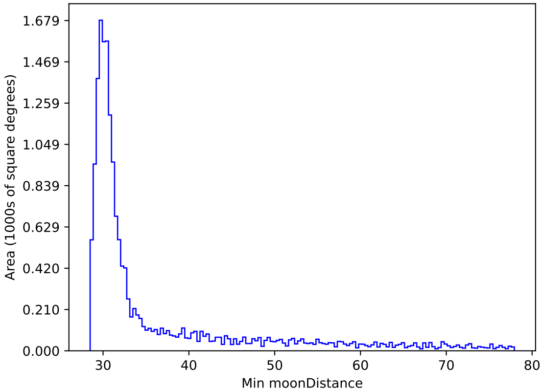
noroll_mjdp60_v3.4_10yrs WFD i band: Min moonDistance
