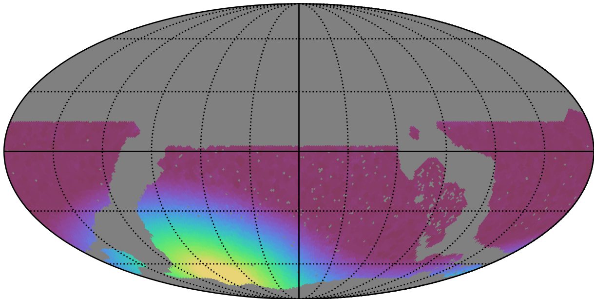
noroll_mjdp60_v3.4_10yrs WFD all bands: Min moonDistance
