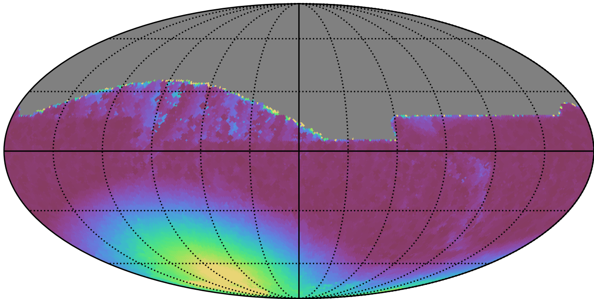
noroll_mjdp60_v3.4_10yrs All sky z band: Min moonDistance
